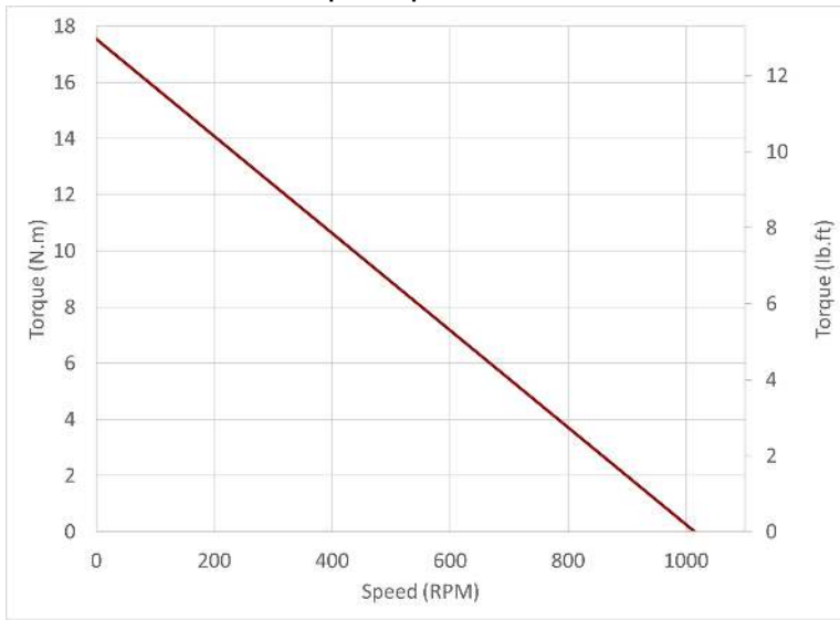
Torque-Speed Curve
