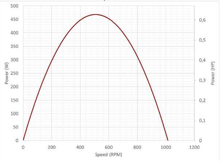
Power-Speed Curve
