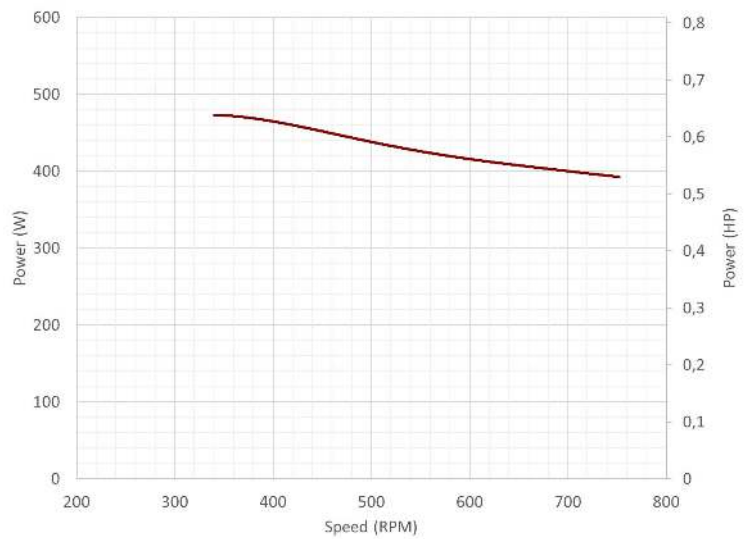
Power-Speed Curve
