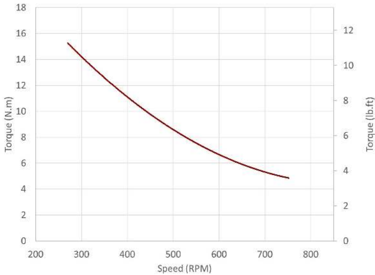
Torque-Speed Curve
